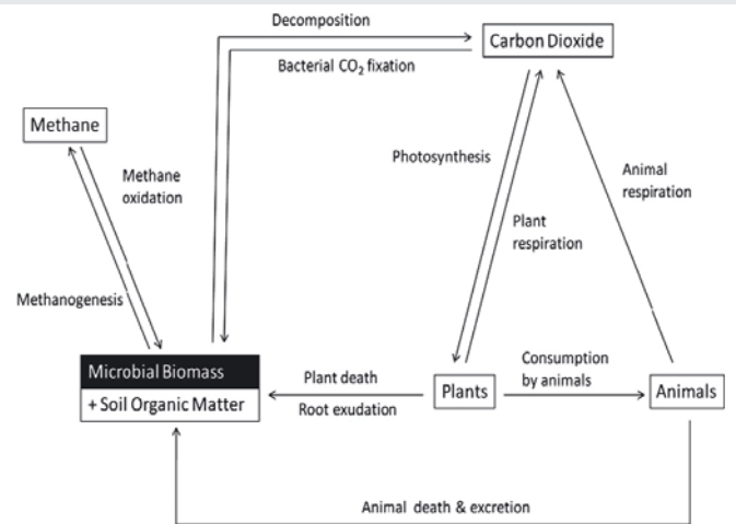
Figure 1: The terrestrial carbon cycle with the major processes mediated by soil microorganisms.
