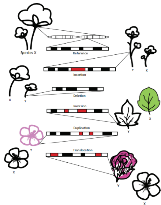
Figure 1: Conceptual representation of different genomic structural variations to a single region of the reference genome.
