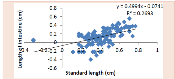
Figure 8: Diagram of relationship between length of intestine and standard length of Stomatorhinus cf polli .
